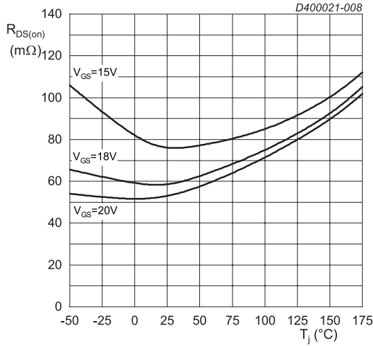
I_{DS} = 20 \text{ A}; t_p < 200 \mu\text{s} Fig. 8. Drain-source on-state resistance as a function of junction temperature
